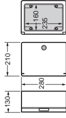
Armario / Enclosure - Ref. Item 39123-T / 39123
