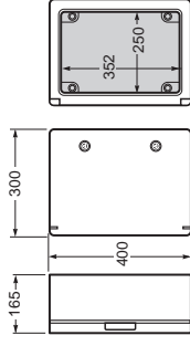
Armario / Enclosure - Ref. Item 39134-T / 39134
