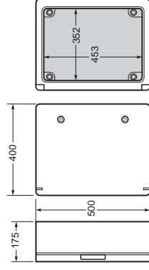
Armario / Enclosure - Ref. Item 39145-T / 39145
