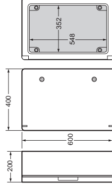
Armario / Enclosure - Ref. Item 39146-T / 39146
