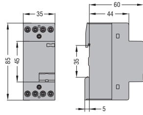
CN25... - CN32... (3-polig - 4-polig)
