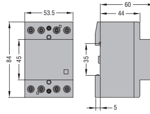
CN40... - CN63... (3-polig - 4-polig)
