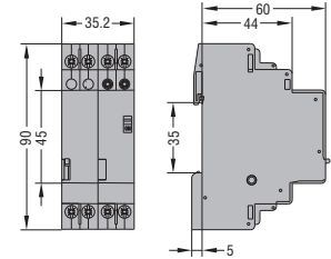
SCHRITTSCHALTER CNB... CNB20... - CNB32... (1-polig - 2-polig) CNB32... (3-polig - 4-polig)
